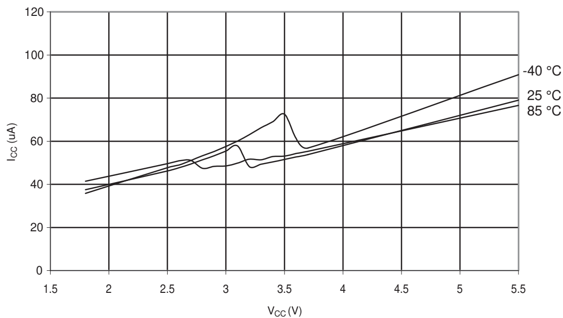
Figure 29-178. ATmega328P: Analog Comparator Current vs. V_{CC}
