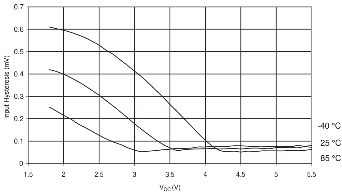
Figure 29-168. ATmega328P: Reset Pin Input Hysteresis vs. V_{CC}
