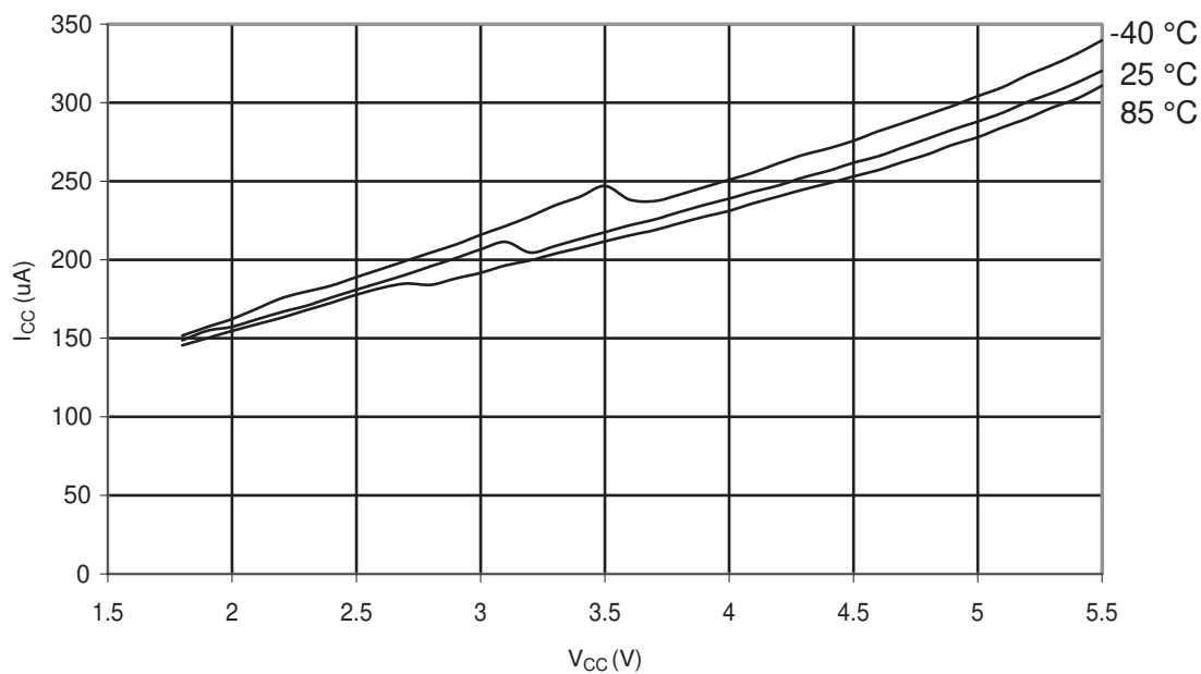
Figure 29-177. ATmega328P: ADC Current vs. V_{CC} (AREF = AV_{CC} )
