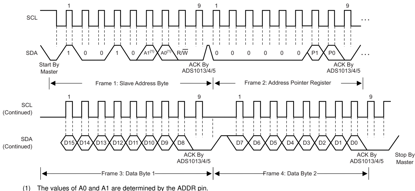
Figure 16. Timing Diagram for Writing to ADS101x
