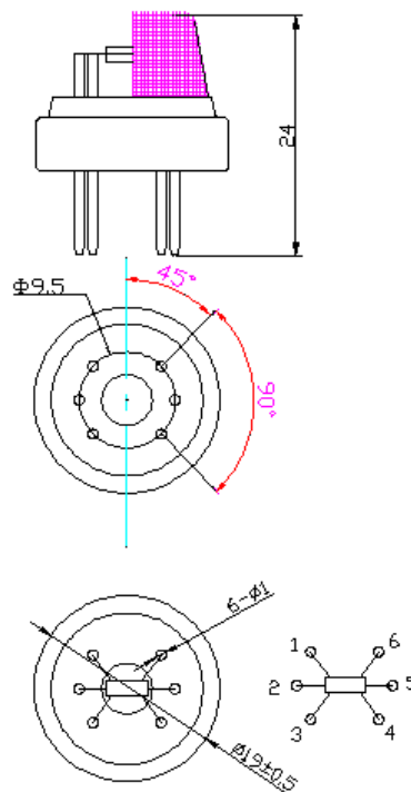
Fig1.Sensor Structure
