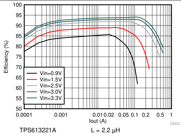
Figure 3. Load Efficiency with Different Inputs
